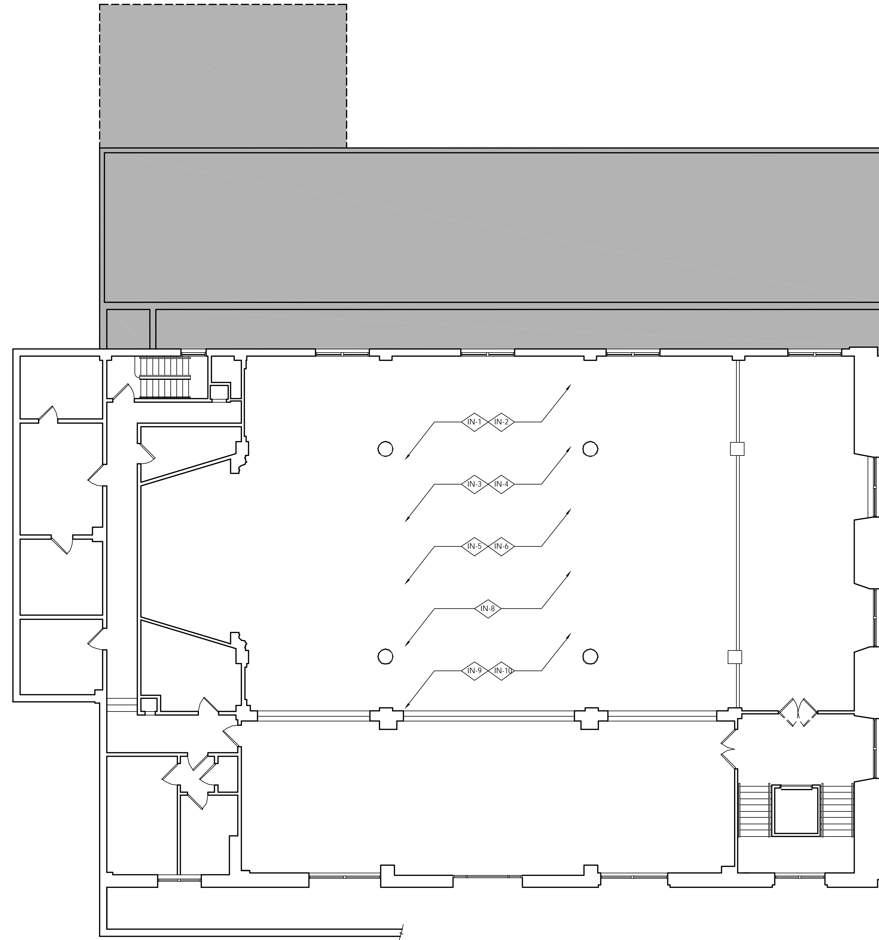
EXISTING SECOND FLOOR MEZZANINE PLAN SCALE: 0 4' 8' 16'
