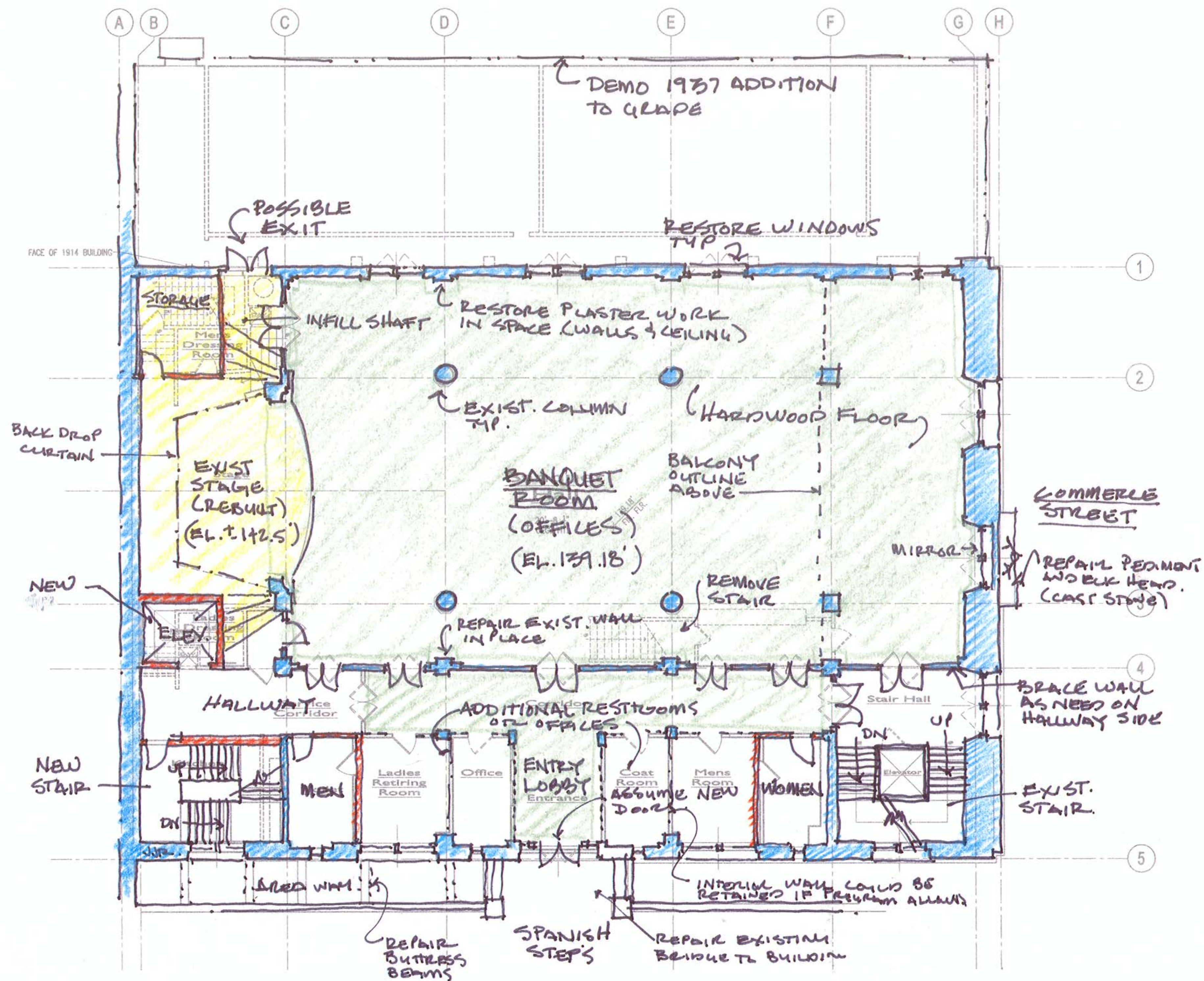
A SECOND FLOOR PLAN - BANQUET HALL LEVEL
