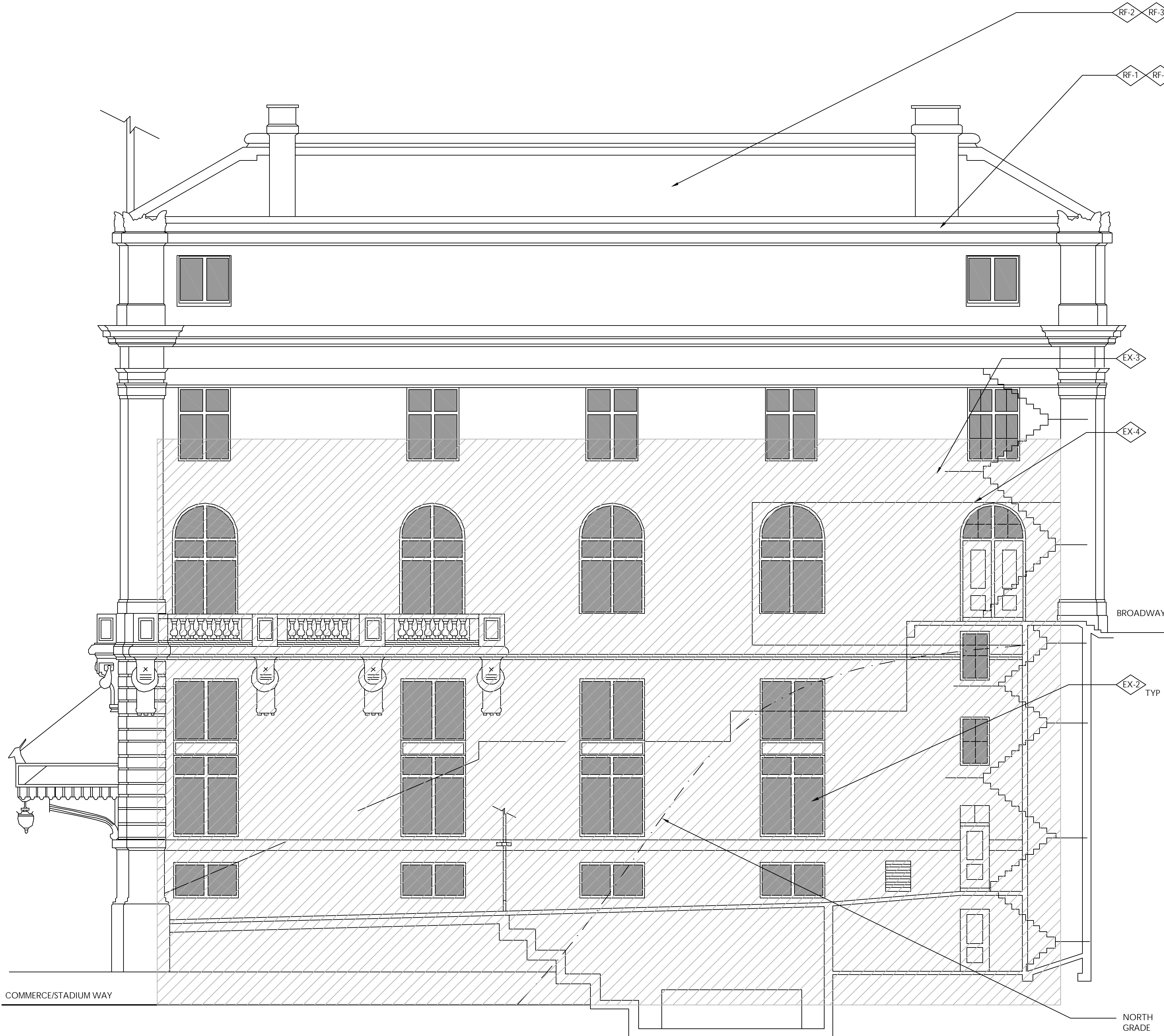
1 NORTH ELEVATION SCALE: 0 4' 8' 16'
