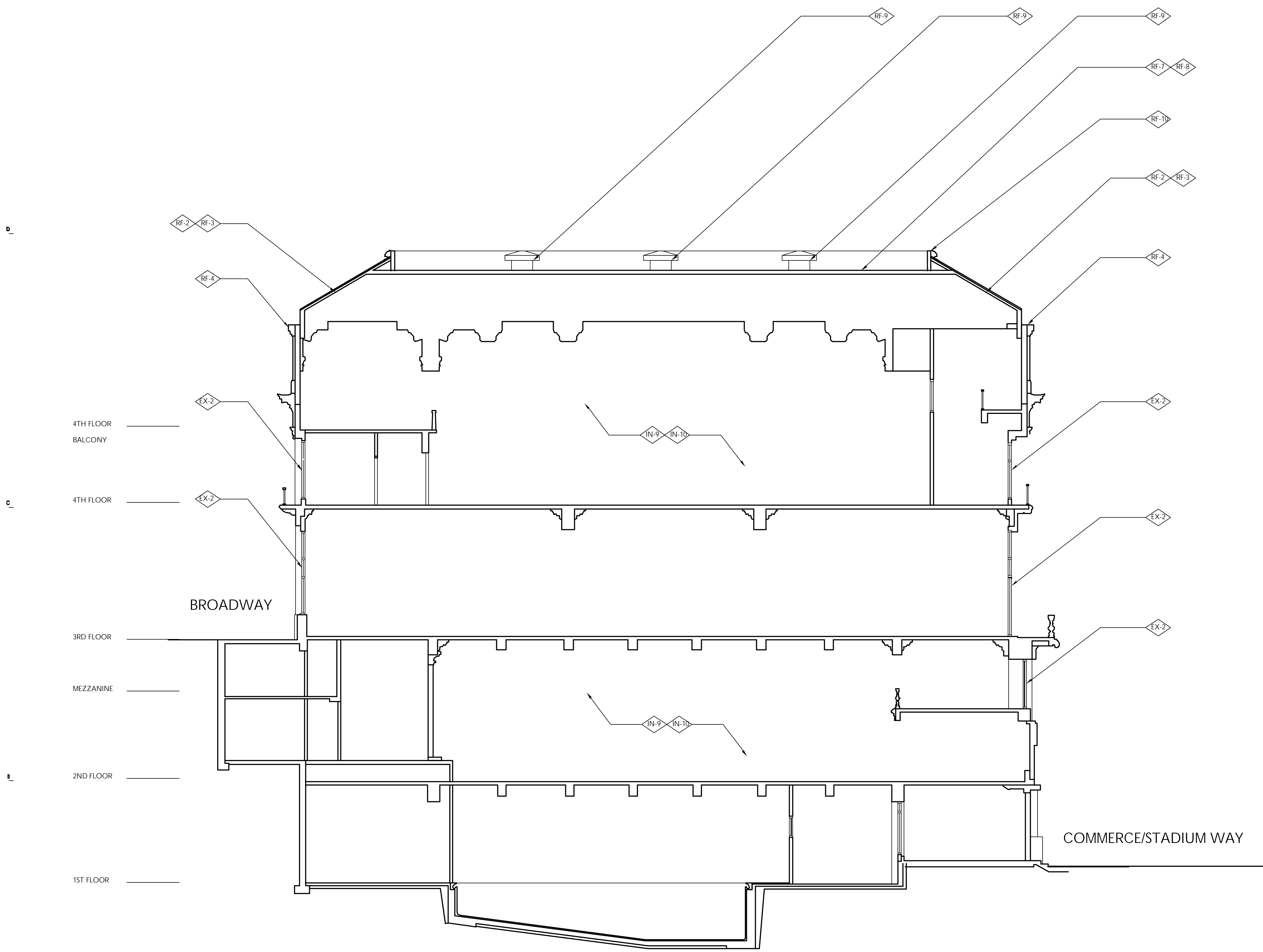
I LONGITUDINAL SECTION (LOOKING NORTH) SCALE: 1/8" = 1'-0"
